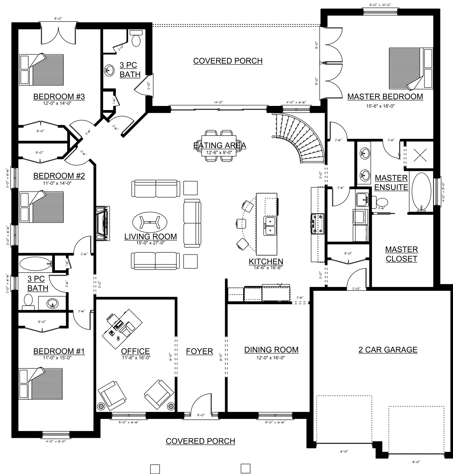
MAIN FLOOR PLAN: 3006.1 Sqft
