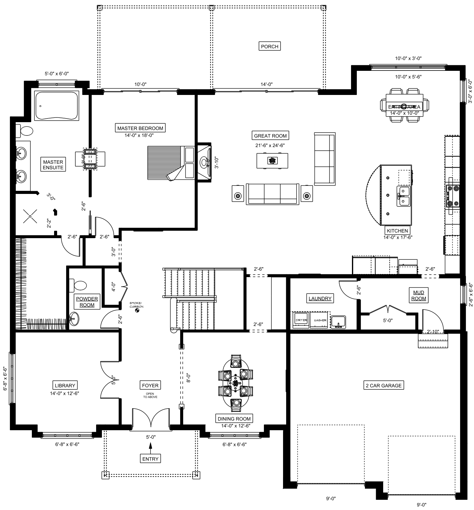
MAIN FLOOR 2545.1 Sqft
